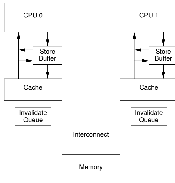
Figure C.7: Caches With Invalidation Queues
