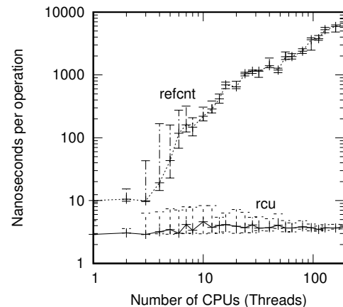
Figure 9.28: Performance of Preemptible RCU vs. Reference Counting
