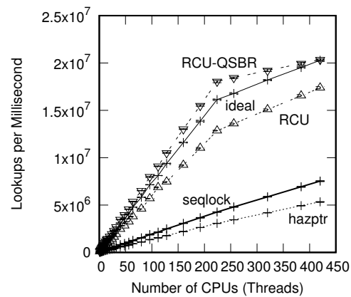
Figure 9.22: Pre-BSD Routing Table Protected by RCU QSBR
