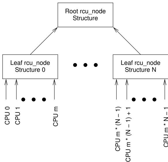
Figure 7.9: Locking Hierarchy
