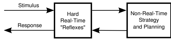
Figure 14.4: Real-Time Reflexes
