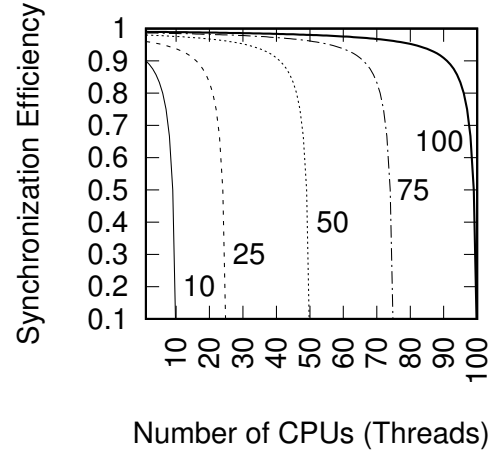
Figure 6.16: Synchronization Efficiency
